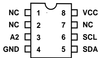
8 pin PDIP
